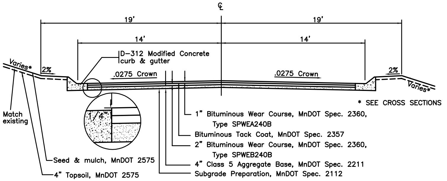
TYPICAL URBAN SECTION
