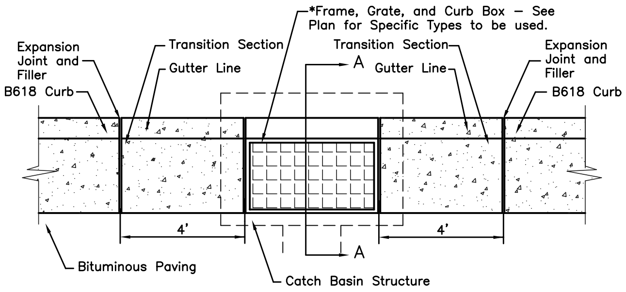
CATCH BASIN PLAN
